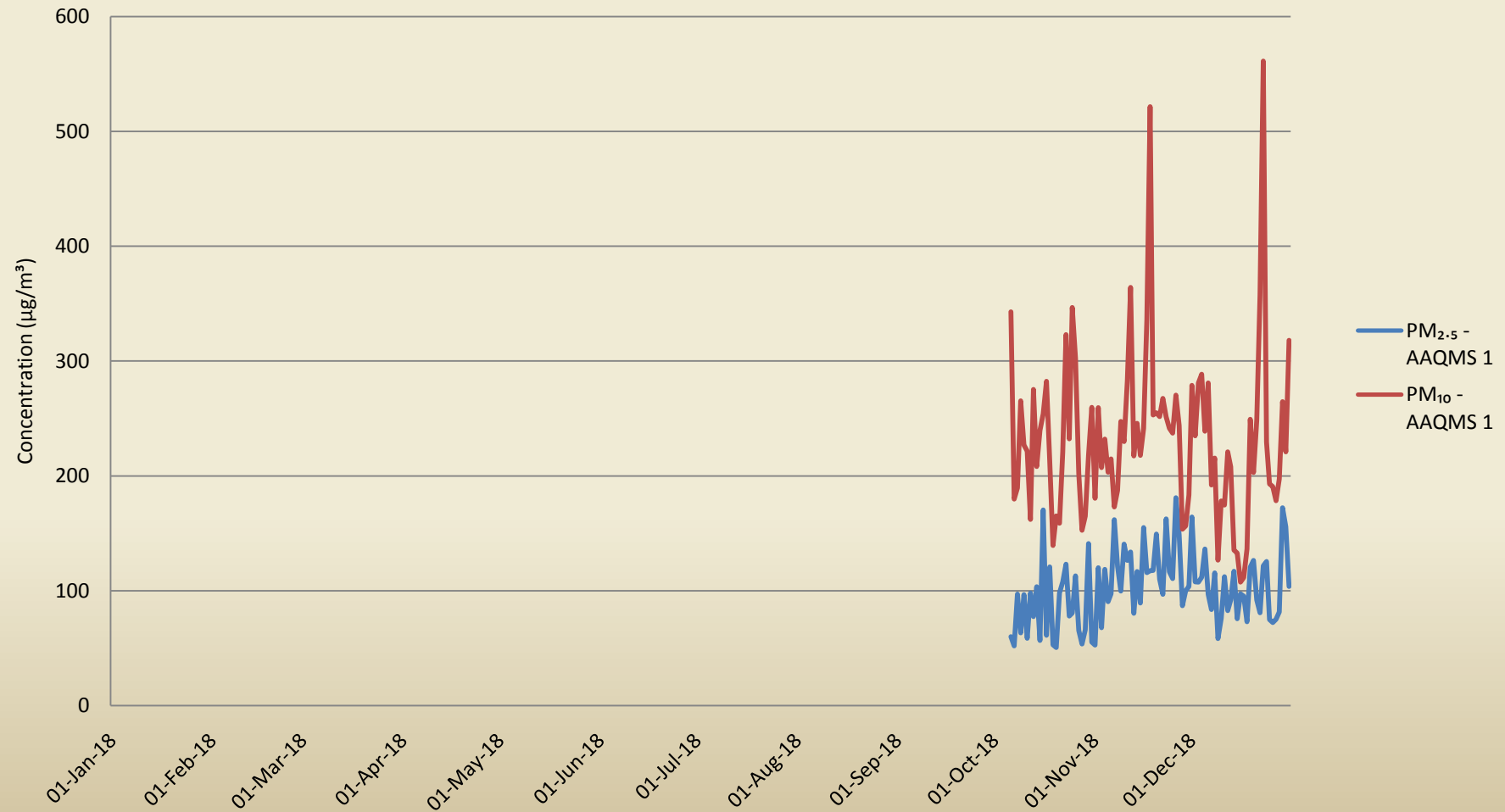
Annual Ambient Trend of Particulate Matter in M/s. Vardhaman Yarns, Dist. Raisen (M.P.)
